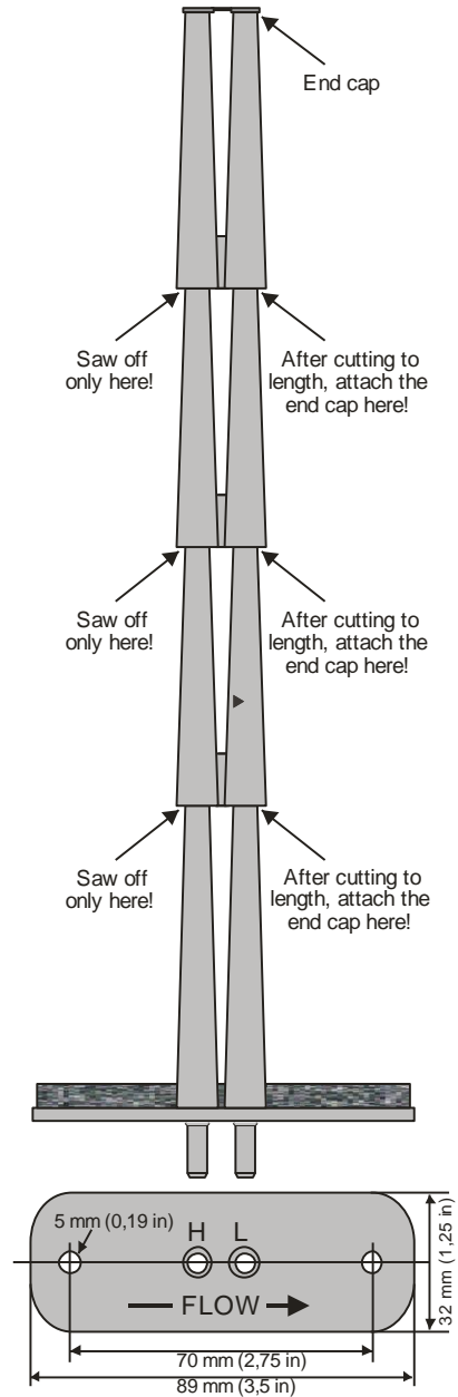
Sampling tube
